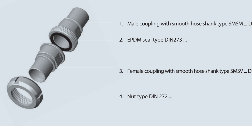
Food couplings SMS 1145 vs DIN 11851
